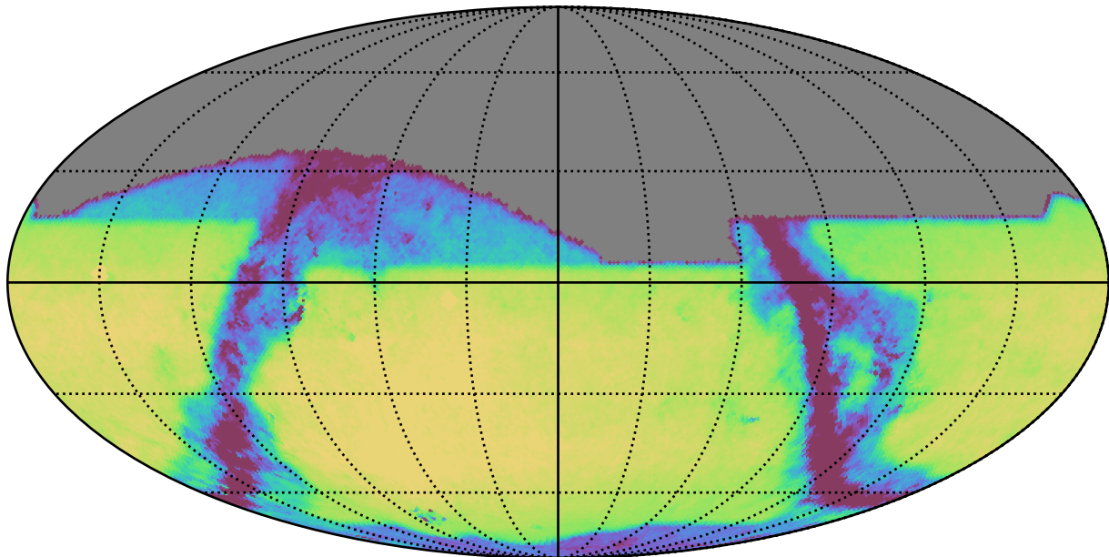
early_u_fpextra4.0_v3.4_10yrs All sky z band: Exgal_CoaddM5
