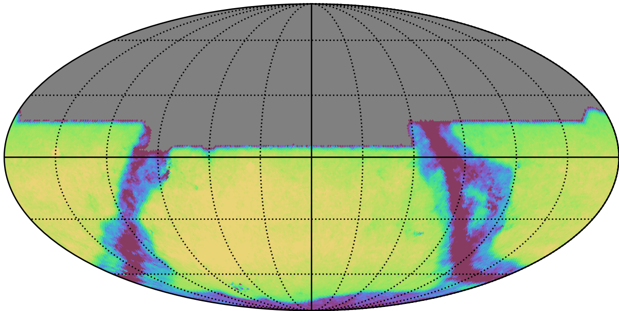
early_u_fpextra4.0_v3.4_10yrs All sky y band: Exgal_CoaddM5
