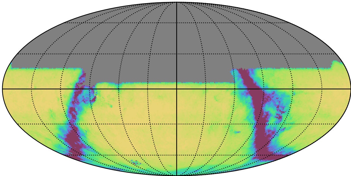
early_u_fpextra4.0_v3.4_10yrs All sky u band: Exgal_CoaddM5
