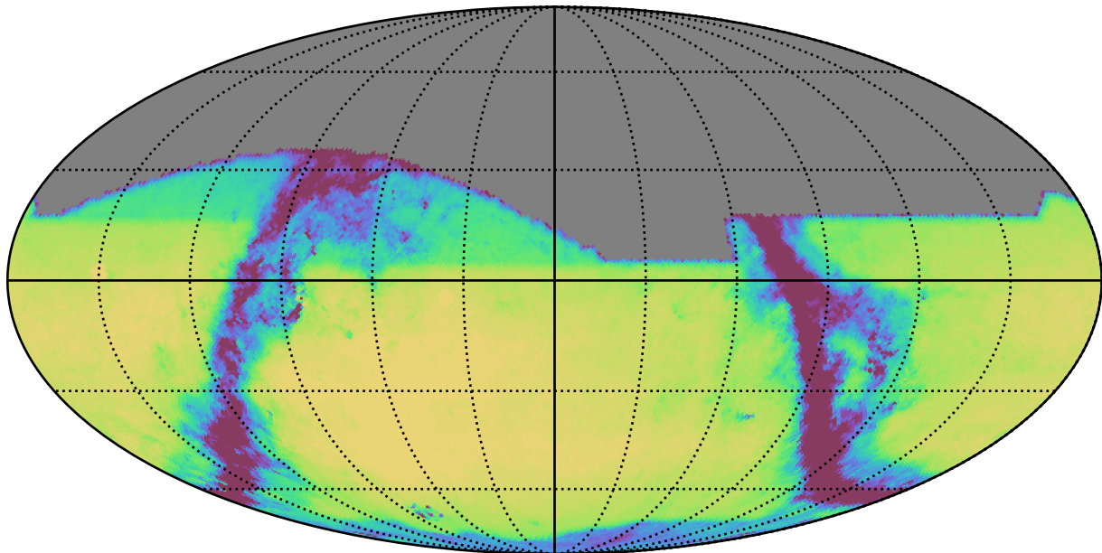
early_u_fpextra4.0_v3.4_10yrs All sky r band: Exgal_CoaddM5
