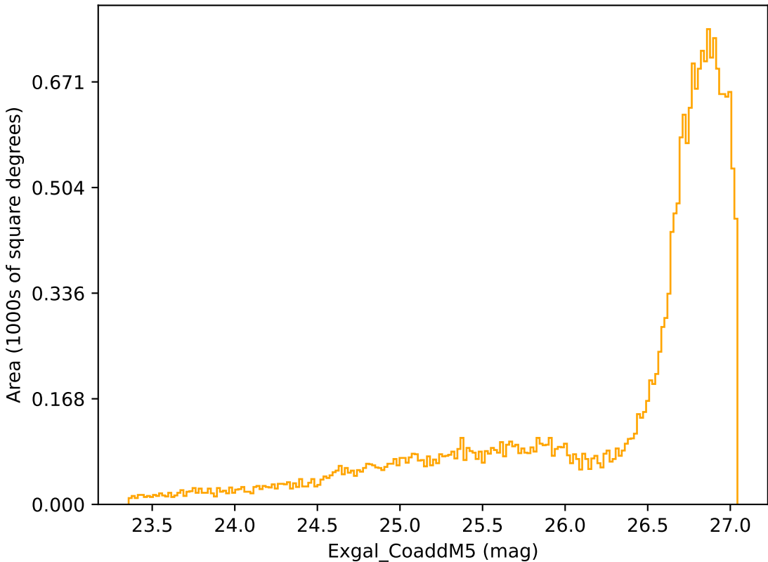
early_u_fpextra4.0_v3.4_10yrs All sky r band: Exgal_CoaddM5
