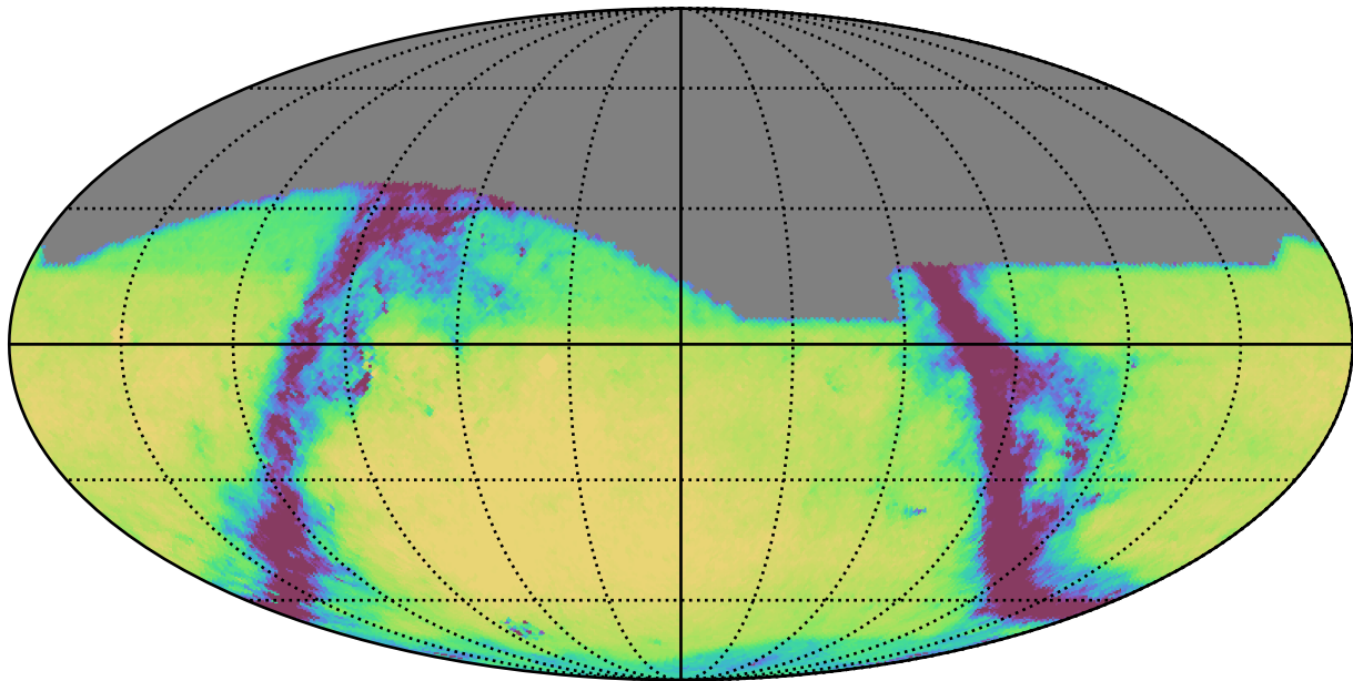
early_u_fpextra4.0_v3.4_10yrs All sky g band: Exgal_CoaddM5
