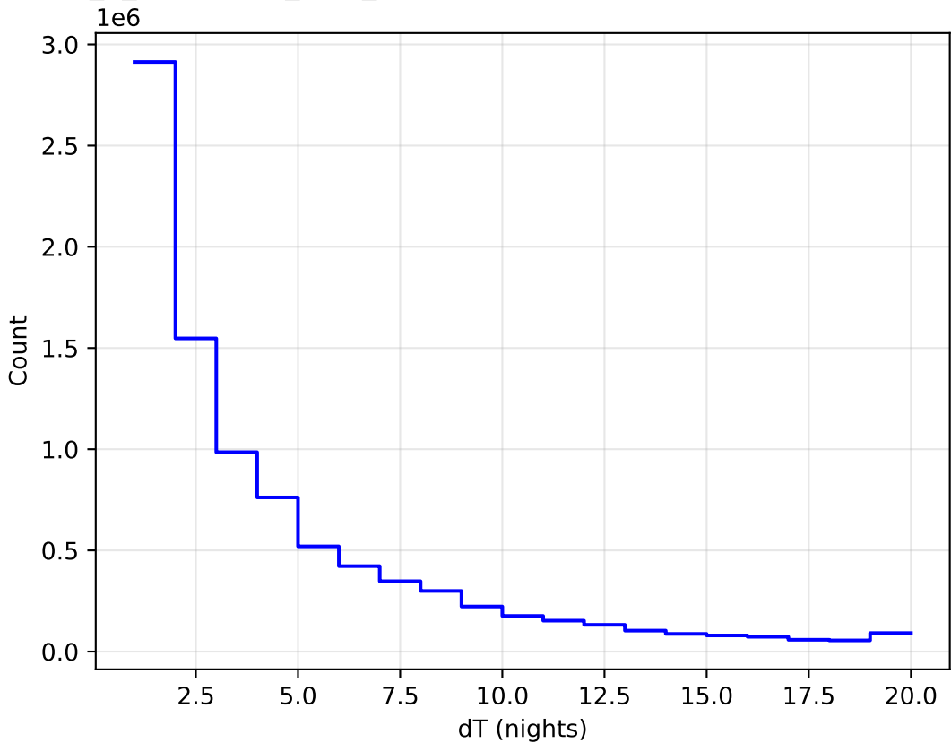
early_u_fpextra4.0_v3.4_10yrs All sky all bands: DeltaNight Histogram
