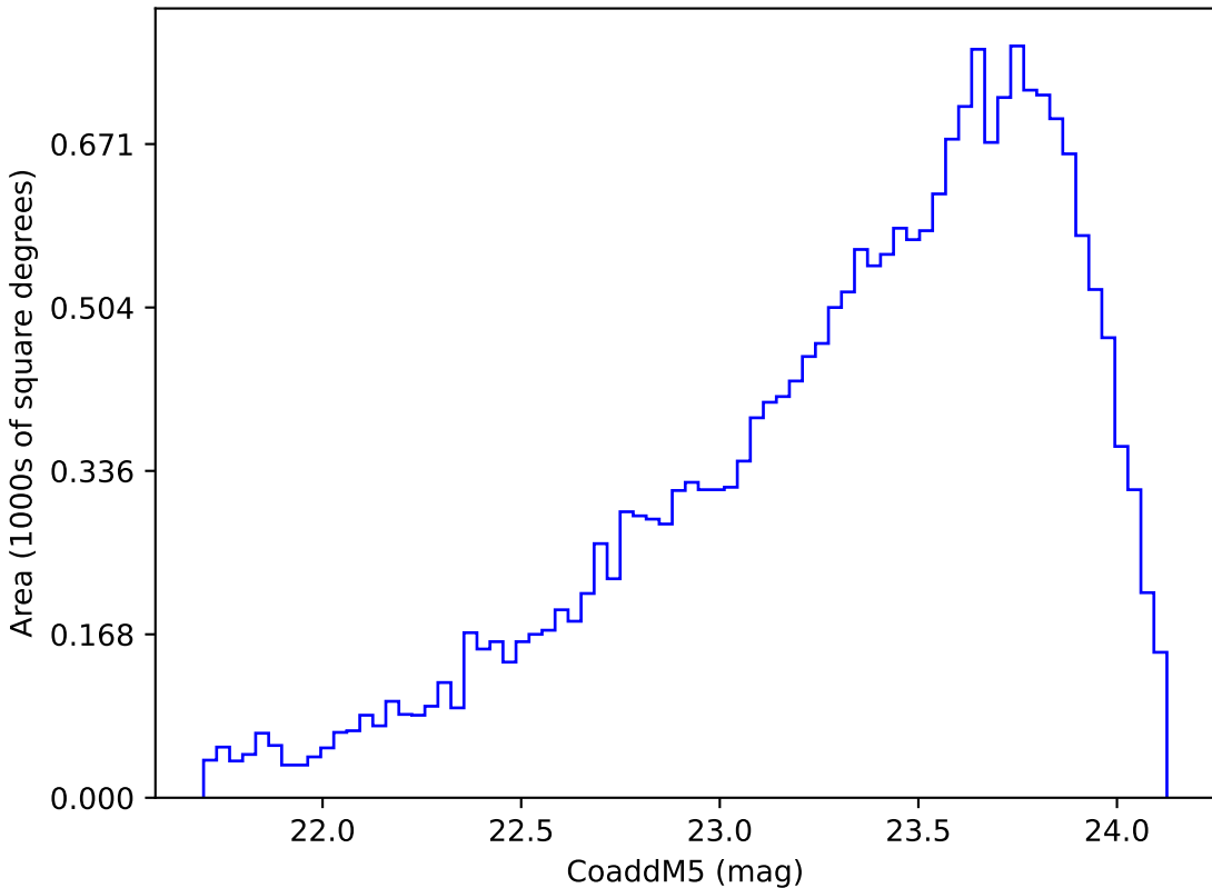
early_u_fpextra4.0_v3.4_10yrs Yr 3-4 y band: CoaddM5
