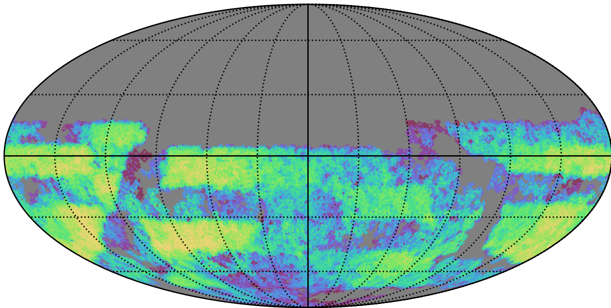
early_u_fpextra4.0_v3.4_10yrs Yr 3-4 u band: CoaddM5
