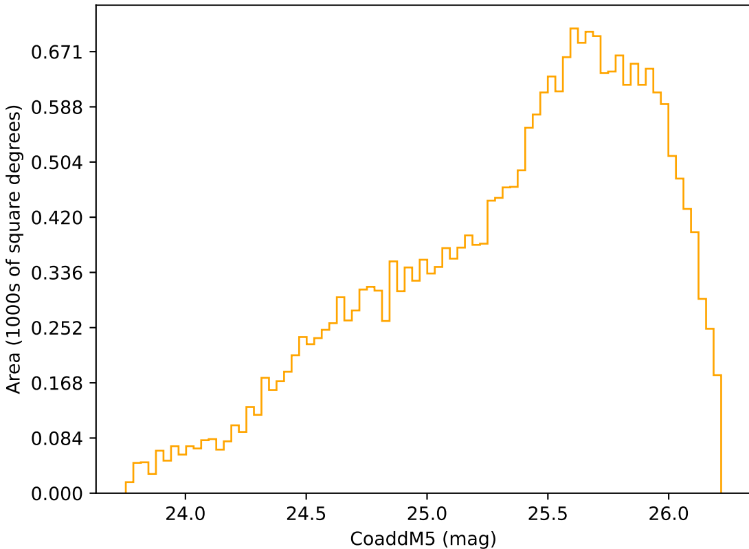
early_u_fpextra4.0_v3.4_10yrs Yr 3-4 r band: CoaddM5
