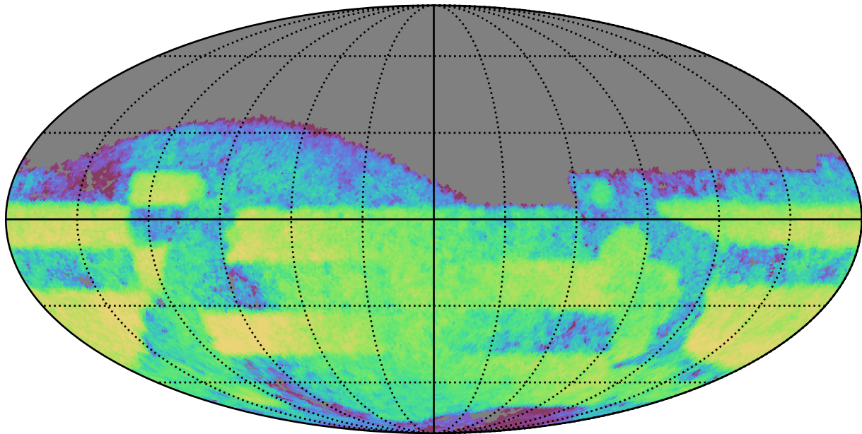
early_u_fpextra4.0_v3.4_10yrs Yr 3-4 i band: CoaddM5
