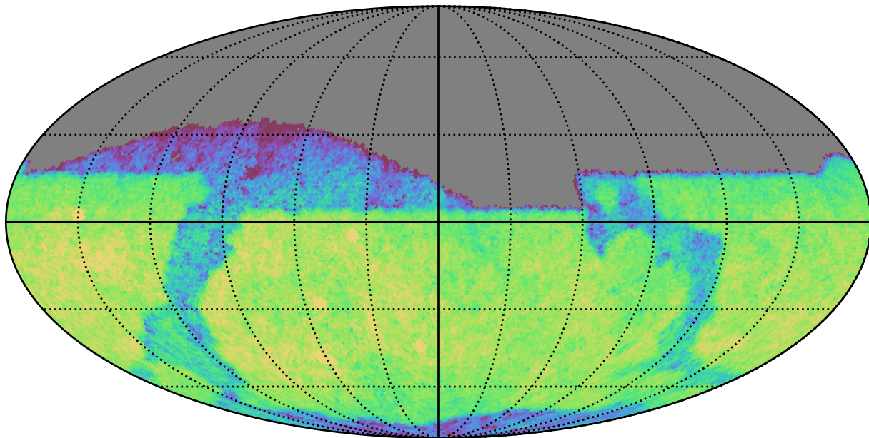
early_u_fpextra4.0_v3.4_10yrs Yr 1 z band: CoaddM5
