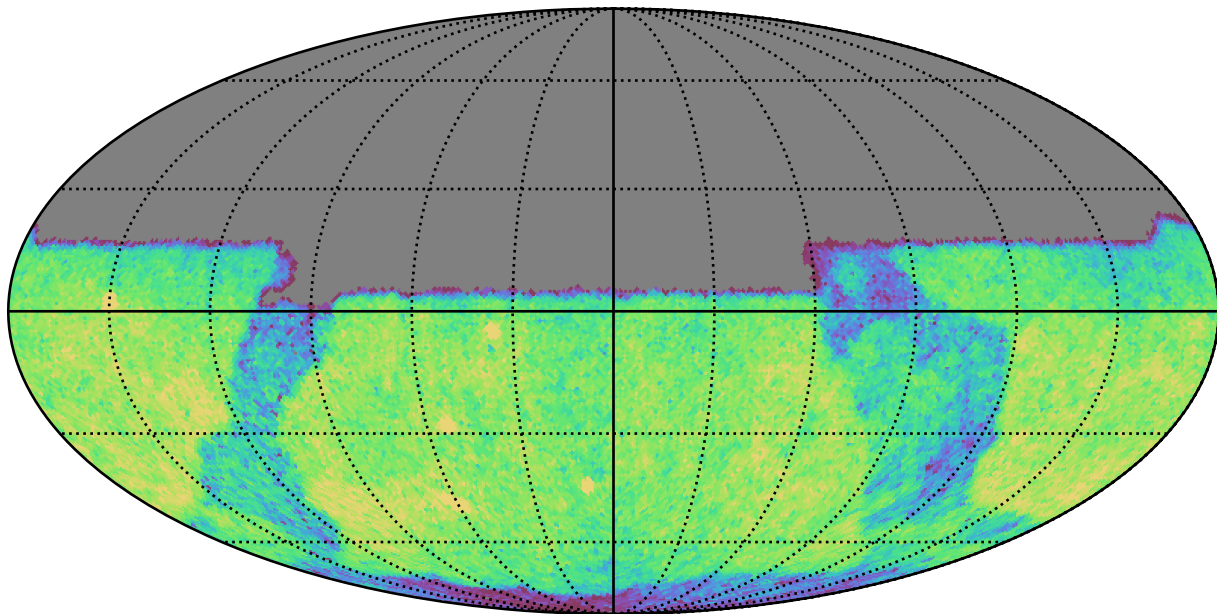
early_u_fpextra4.0_v3.4_10yrs Yr 1 y band: CoaddM5
