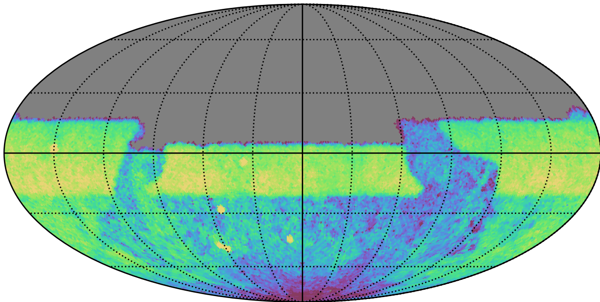
early_u_fpextra4.0_v3.4_10yrs Yr 1 u band: CoaddM5
