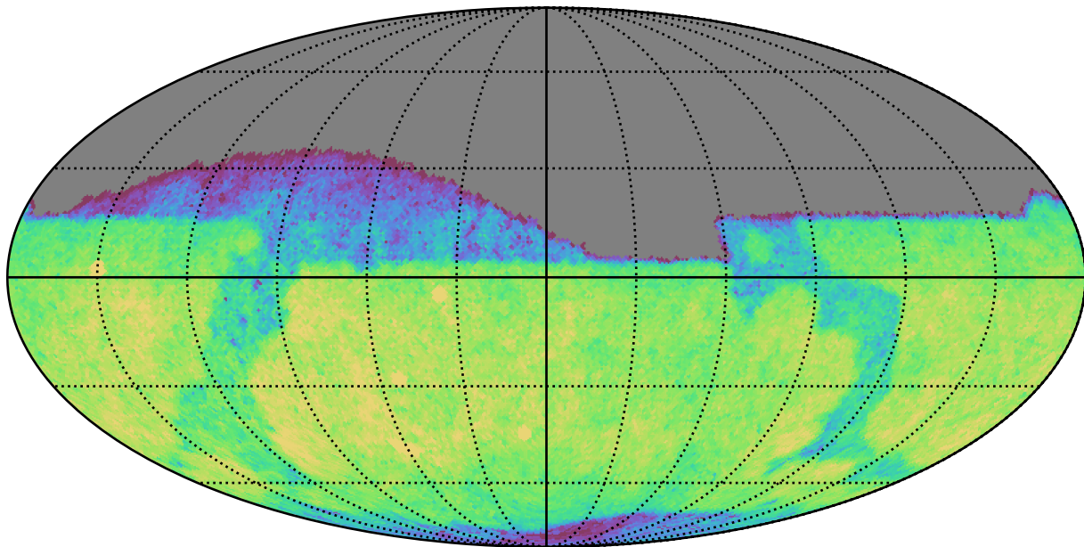
early_u_fpextra4.0_v3.4_10yrs Yr 1 r band: CoaddM5
