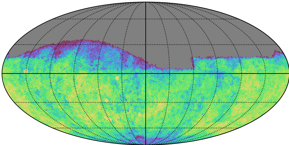
early_u_fpextra4.0_v3.4_10yrs Yr 1 g band: CoaddM5
