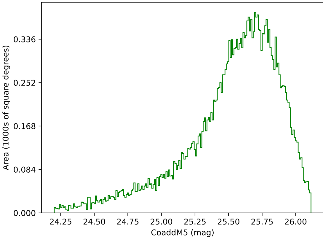
early_u_fpextra4.0_v3.4_10yrs Yr 1 g band: CoaddM5
