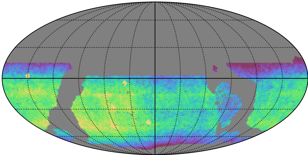
early_u_fpextra4.0_v3.4_10yrs WFD z band: CoaddM5
