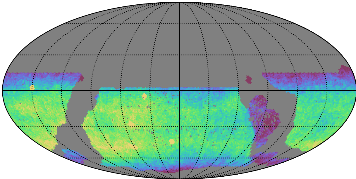
early_u_fpextra4.0_v3.4_10yrs WFD y band: CoaddM5
