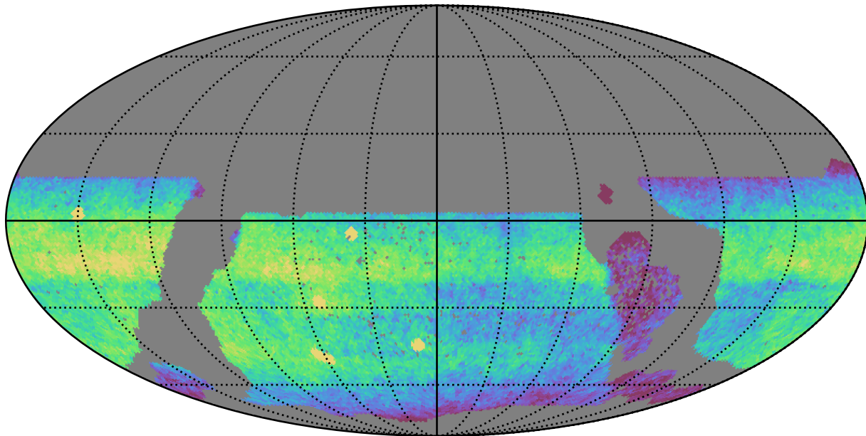
early_u_fpextra4.0_v3.4_10yrs WFD u band: CoaddM5
