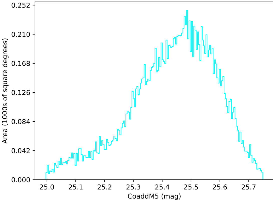
early_u_fpextra4.0_v3.4_10yrs WFD u band: CoaddM5
