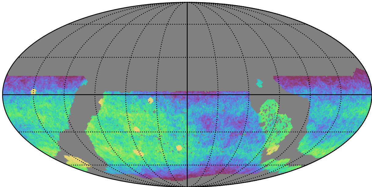
early_u_fpextra4.0_v3.4_10yrs WFD g band: CoaddM5
