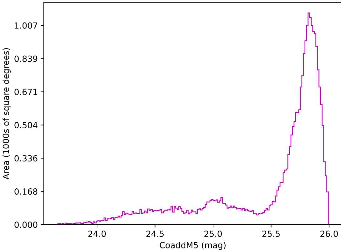
early_u_fpextra4.0_v3.4_10yrs All sky z band: CoaddM5
