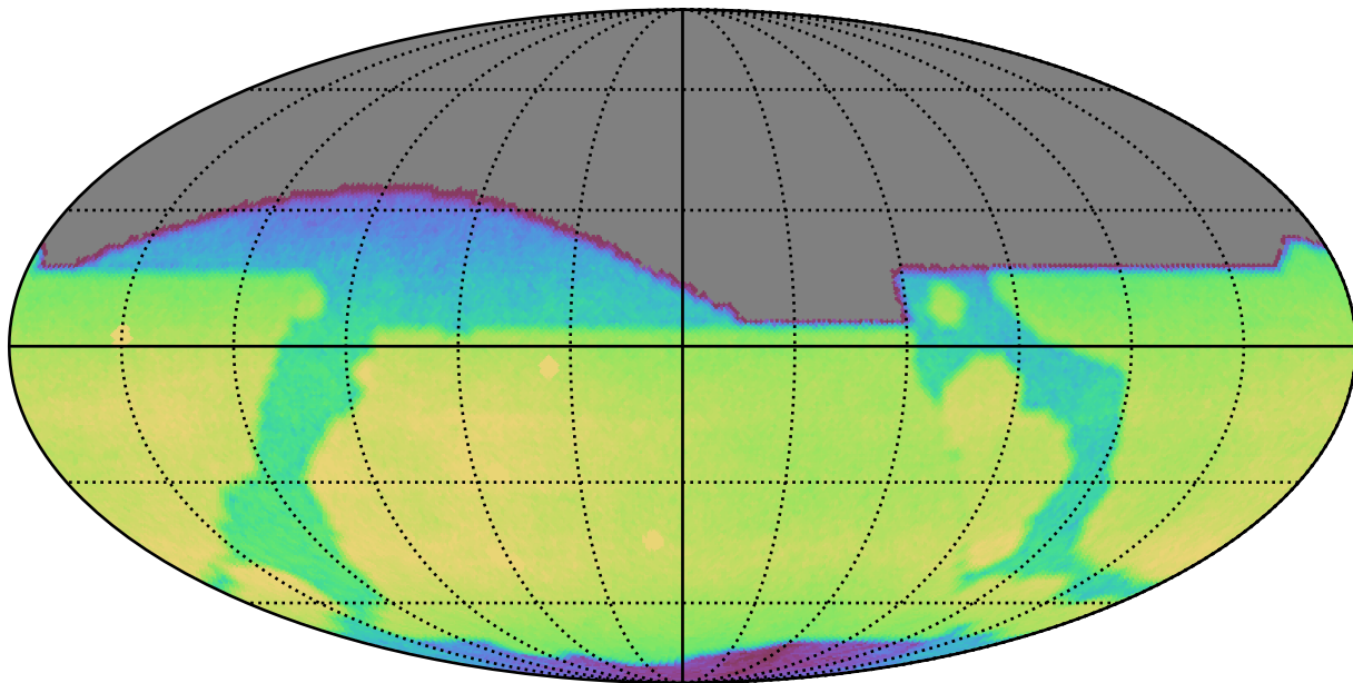
early_u_fpextra4.0_v3.4_10yrs All sky r band: CoaddM5
