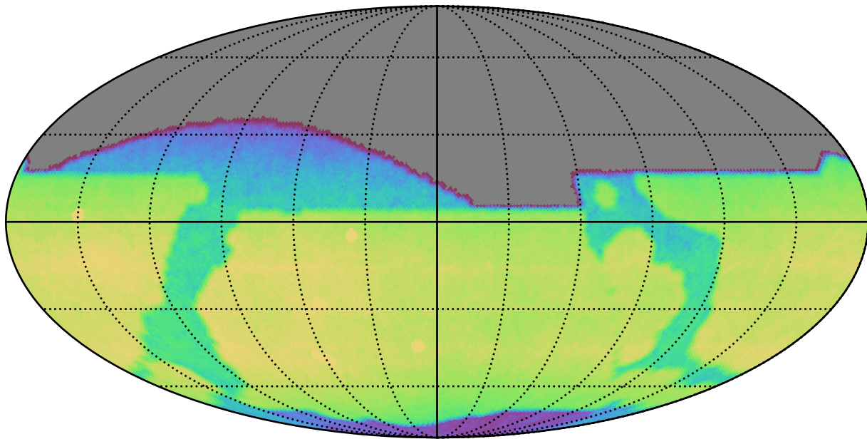
early_u_fpextra4.0_v3.4_10yrs All sky i band: CoaddM5
