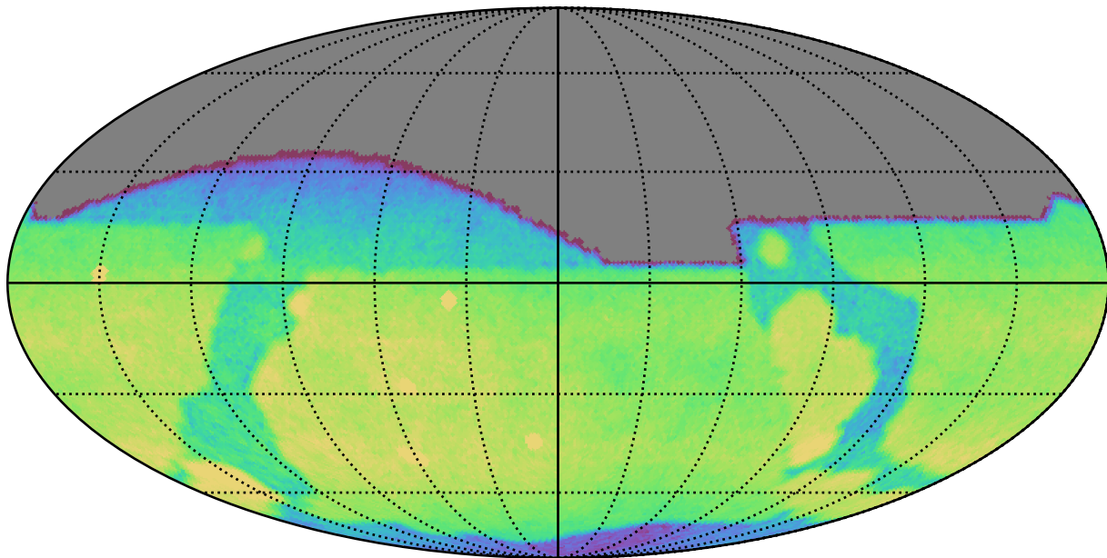
early_u_fpextra4.0_v3.4_10yrs All sky g band: CoaddM5
