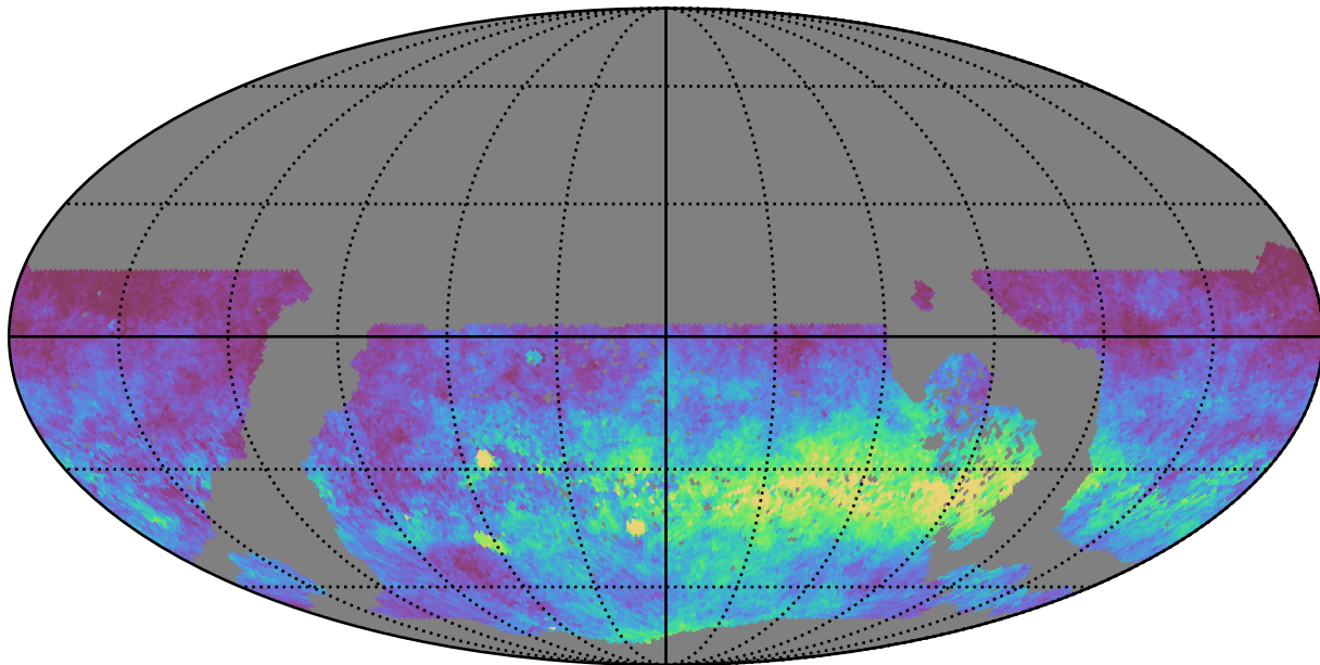
early_u_fpextra4.0_v3.4_10yrs WFD y band: AngleRms rotSkyPos
