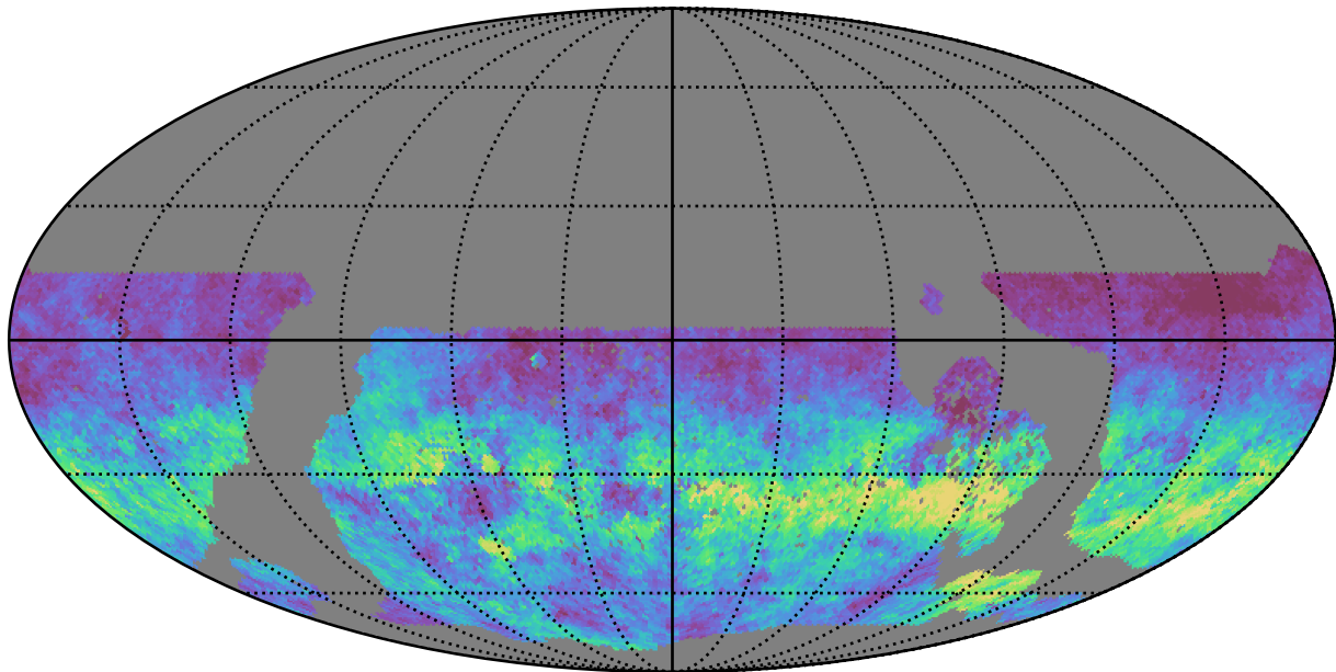
early_u_fpextra4.0_v3.4_10yrs WFD u band: AngleRms rotSkyPos
