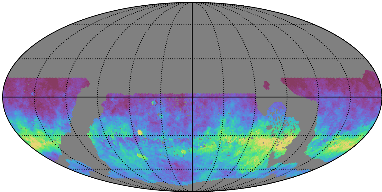
early_u_fpextra4.0_v3.4_10yrs WFD i band: AngleRms rotSkyPos
