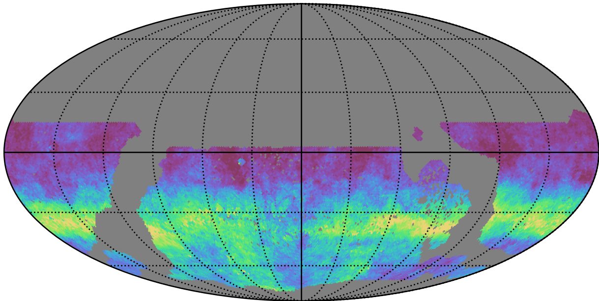
early_u_fpextra4.0_v3.4_10yrs WFD g band: AngleRms rotSkyPos
