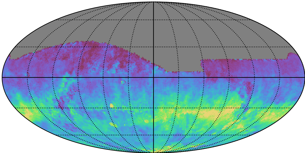
early_u_fpextra4.0_v3.4_10yrs All sky z band: AngleRms rotSkyPos
