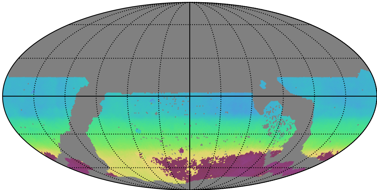
early_u_fpextra4.0_v3.4_10yrs WFD all bands: AngleMean rotSkyPos
