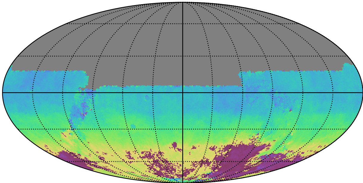
early_u_fpextra4.0_v3.4_10yrs All sky u band: AngleMean rotSkyPos
