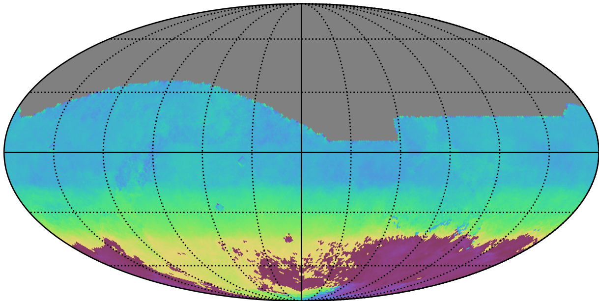
early_u_fpextra4.0_v3.4_10yrs All sky r band: AngleMean rotSkyPos
