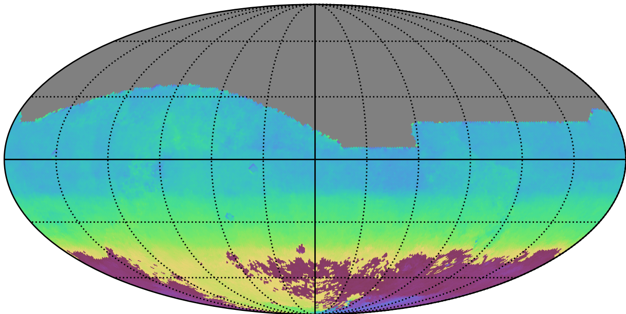
early_u_fpextra4.0_v3.4_10yrs All sky i band: AngleMean rotSkyPos
