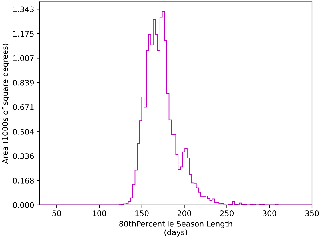
early_u_fpextra4.0_v3.4_10yrs WFD z band: 80thPercentile Season Length
