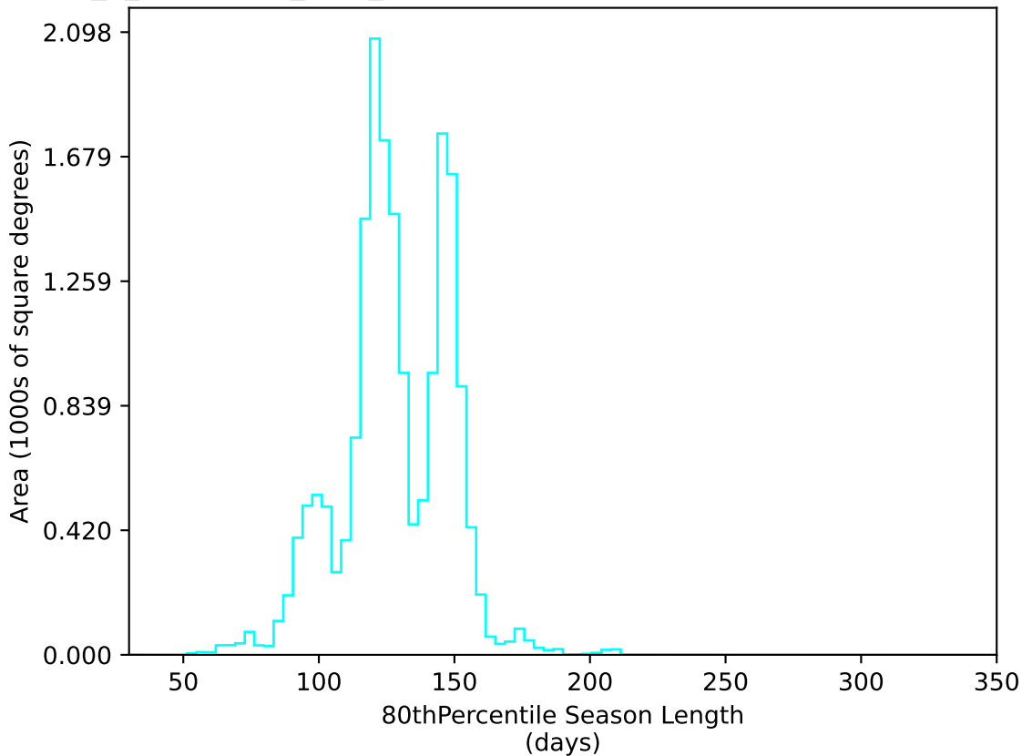
early_u_fpextra4.0_v3.4_10yrs WFD u band: 80thPercentile Season Length
