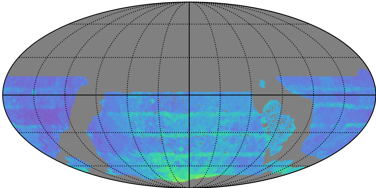
early_u_fpextra4.0_v3.4_10yrs WFD all bands: 80thPercentile Season Length
