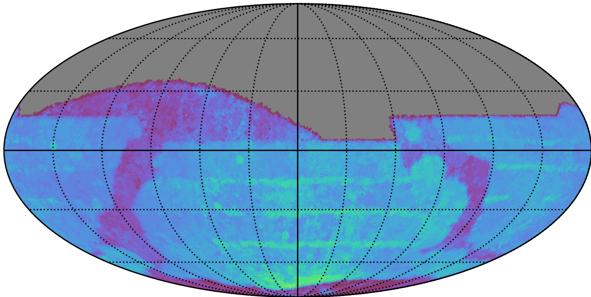
early_u_fpextra4.0_v3.4_10yrs All sky z band: 80thPercentile Season Length
