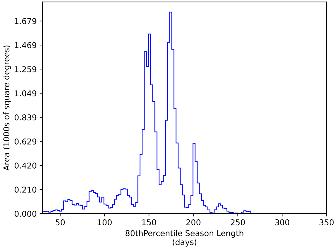
early_u_fpextra4.0_v3.4_10yrs All sky y band: 80thPercentile Season Length
