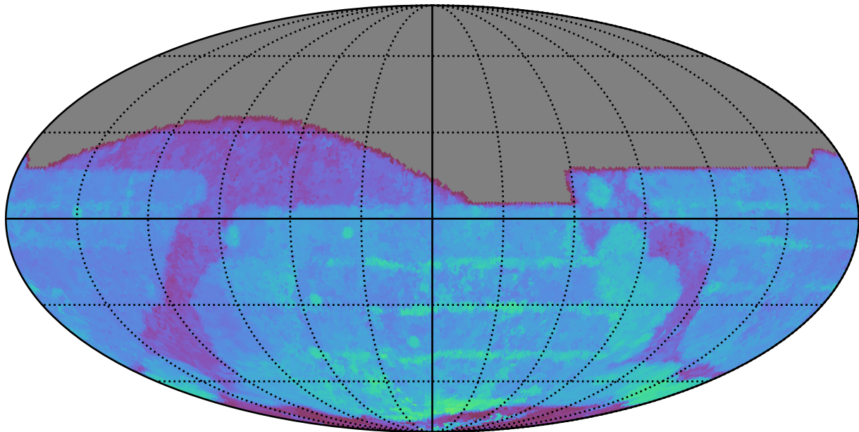
early_u_fpextra4.0_v3.4_10yrs All sky r band: 80thPercentile Season Length
