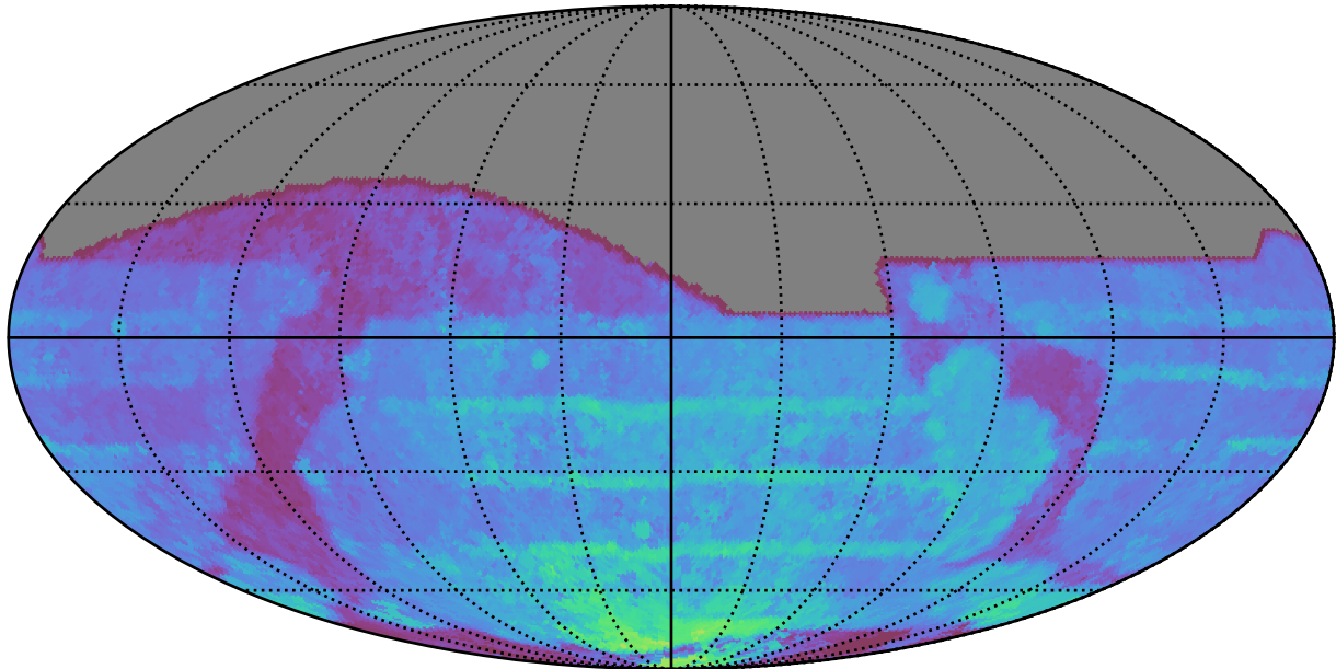
early_u_fpextra4.0_v3.4_10yrs All sky all bands: 80thPercentile Season Length
