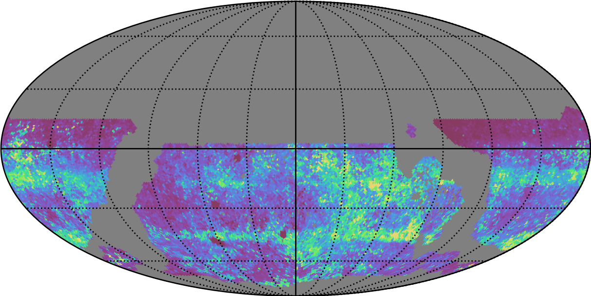
early_u_fpextra4.0_v3.4_10yrs WFD zy bands: 75th Percentile Intranight Timespan
