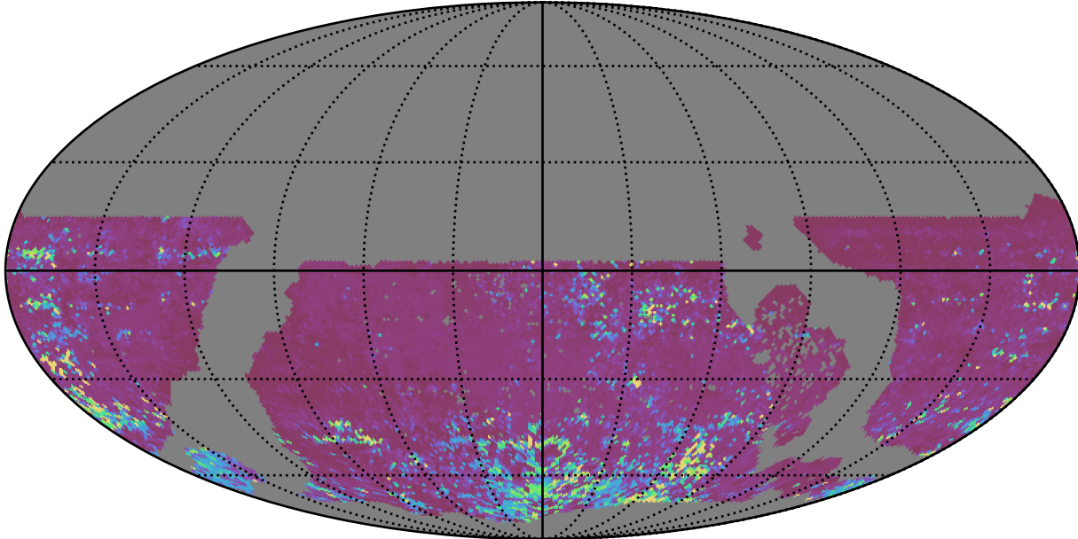
early_u_fpextra4.0_v3.4_10yrs WFD z band: 75th Percentile Intranight Timespan
