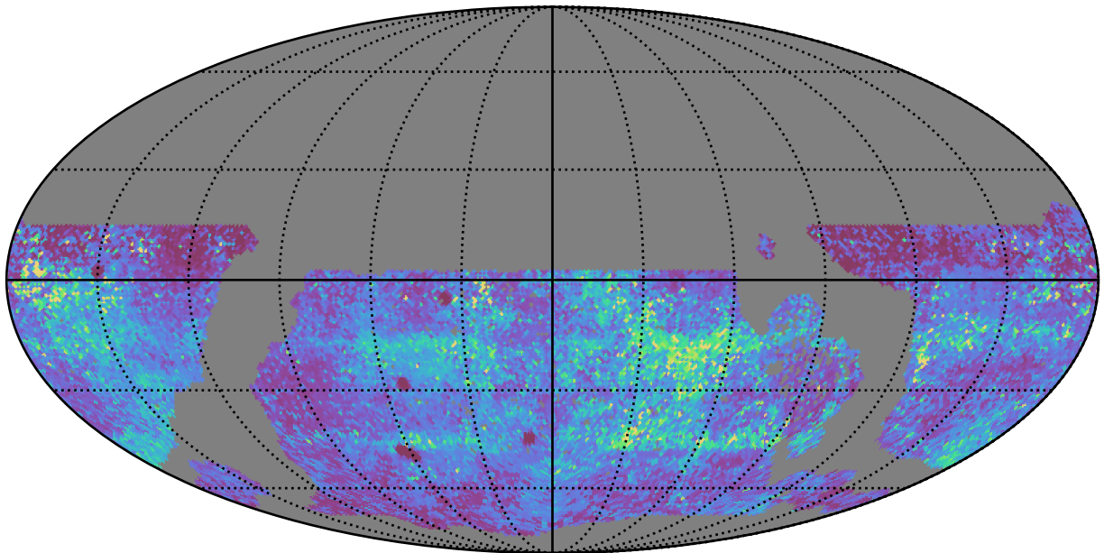
early_u_fpextra4.0_v3.4_10yrs WFD y band: 75th Percentile Intranight Timespan
