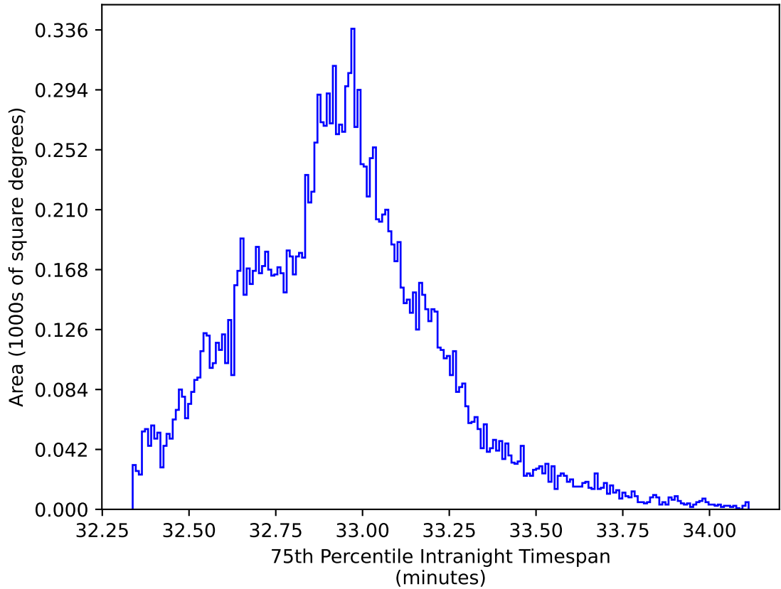
early_u_fpextra4.0_v3.4_10yrs WFD y band: 75th Percentile Intranight Timespan
