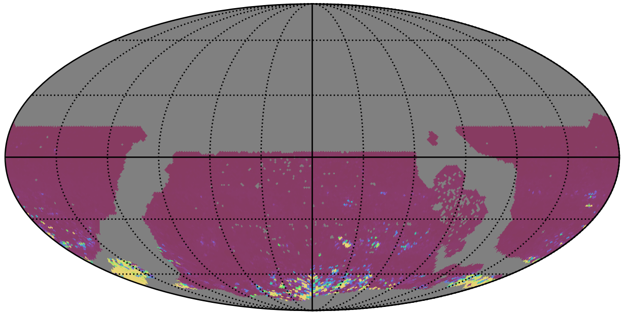
early_u_fpextra4.0_v3.4_10yrs WFD ri bands: 75th Percentile Intranight Timespan
