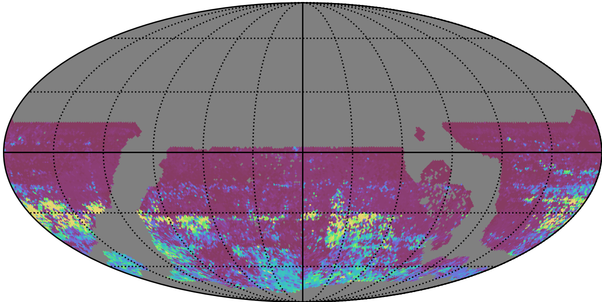
early_u_fpextra4.0_v3.4_10yrs WFD r band: 75th Percentile Intranight Timespan
