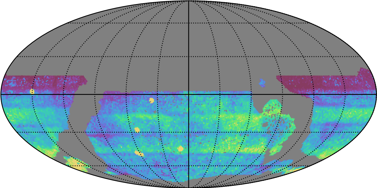
early_u_fpextra4.0_v3.4_10yrs WFD all bands: 75th Percentile Intranight Timespan
