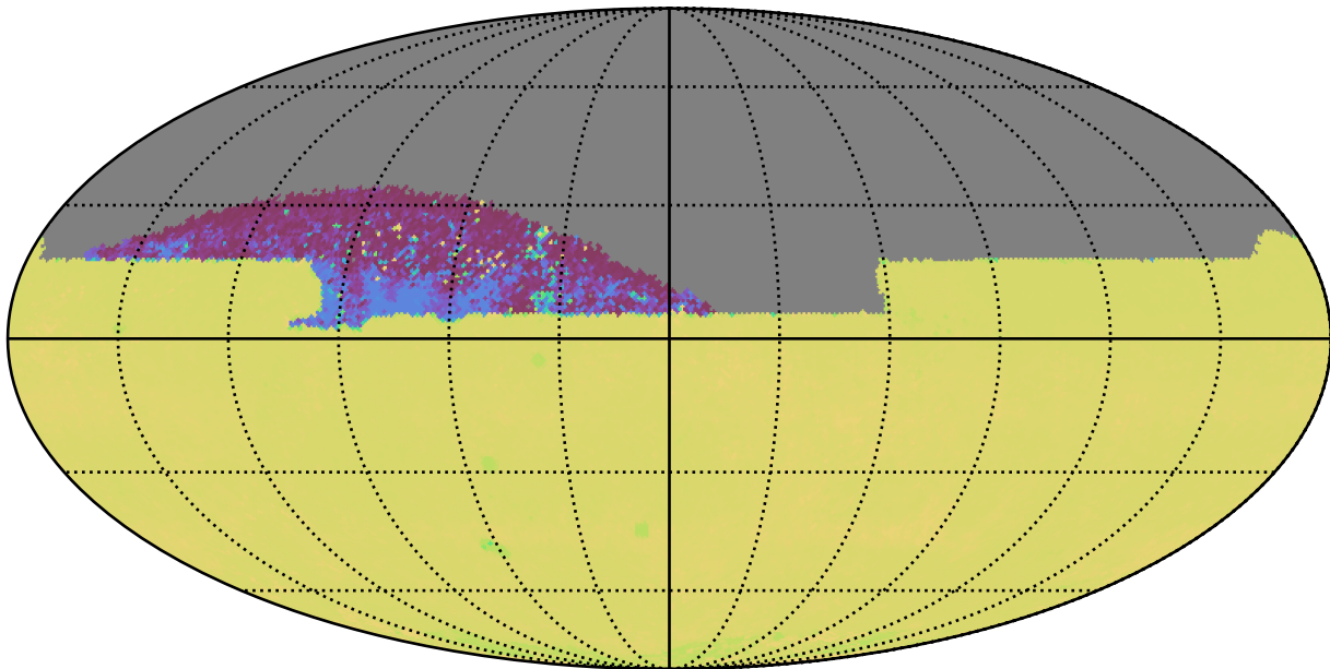
early_u_fpextra4.0_v3.4_10yrs All sky zy bands: 75th Percentile Intranight Timespan
